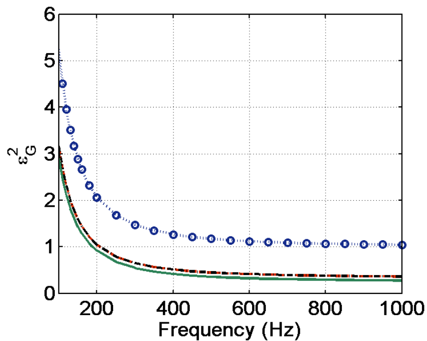
Figure 3.6 Ensemble variance of different GED quantities for a reverberation chamber with V = 136.6 \text{ m}^2 and uniform T_{60} = 6.2 \text{ s} . “ \cdot \cdot \bigcirc \cdot \cdot ” : E_{G(1)} (E_P) ; “ -\ - ” : E_{G(0)} (E_K) ; “ -\cdot - ” : E_{G(1/2)} (E_T) ; “ -\ - ” : E_{G(1/4)} .
