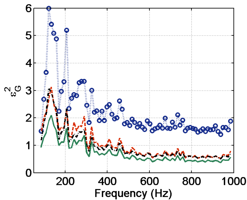
Figure 3.7 Numerical simulation results for the ensemble variance of different GED quantities for a lightly damped room. “ \dots \bigcirc \dots ”: E_{G(1)} (E_P) ; “ --- ”: E_{G(0)} (E_K) ; “ -.- ”: E_{G(1/2)} (E_T) ; “ — ”: E_{G(1/4)} .
