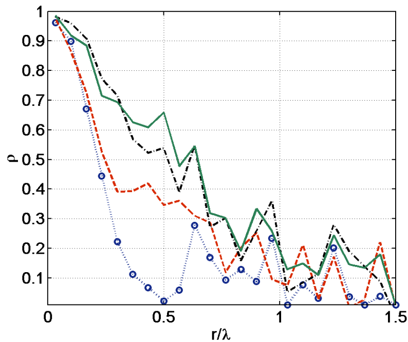
Figure 3.8 Numerical simulation results for the spatial correlation coefficient of GED in a diffuse field. “ \cdot\cdot\bigcirc\cdot\cdot ”: E_{G(1)} (E_P) ; “ -\ - ”: E_{G(0)} (E_K) ; “ -\cdot- ”: E_{G(1/2)} (E_T) ; “ - ”: E_{G(1/4)} .
