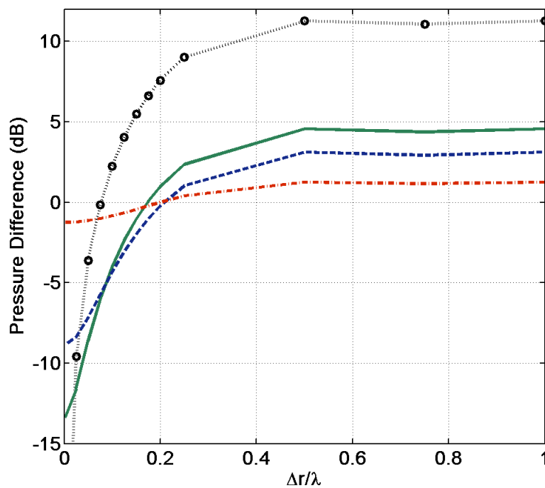
Figure 5.5 Averaged mean square pressure in the near-field of the error sensor when GED is minimized. Eq. (5.16) is evaluated numerically and 10\log(\langle p^2(\mathbf{r}_0 + \Delta\mathbf{r}) \rangle / \langle p_p^2 \rangle) is plotted. “ \cdot\cdot\circ\cdot\cdot ”: E_{G(1)} ( E_P ); “—”: E_{G(0.95)} ; “- -”: E_{G(0.85)} ; “- . -”: E_{G(1/4)} .
