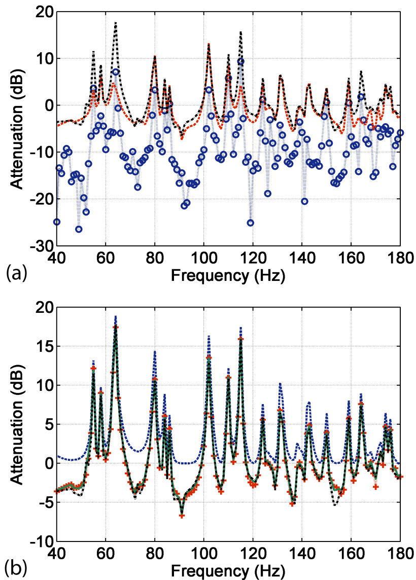
Figure 5.1 Averaged global attenuation using GED-based active noise cancellation in an enclosure with random error sensor locations. (a) Average attenuation based on E_{G(1)} ( E_P , “-○-”), E_{G(0)} ( E_K , “- -”) and E_{G(1/2)} ( E_T , “-.-”). (b) Average attenuation based on E_{G(1/2)} (“-.-”), E_{G(1/4)} (“- -”) and E_{G(1/10)} (“.+.”) with the total potential energy upper-bound limit (“- -”). The attenuation based on total potential energy is considered optimal.
