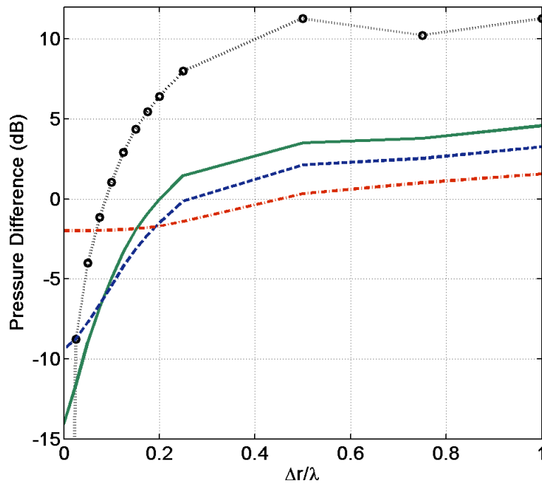
Figure 5.6 Averaged mean square pressure in the near-field of the error sensor when GED is minimized. This is a computer simulation result. “ \cdot \cdot \circ \cdot \cdot ”: E_{G(1)} ( E_P ); “—”: E_{G(0.95)} ; “- -”: E_{G(0.85)} ; “- . -” : E_{G(1/4)} .
